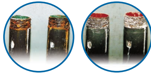
Examples of Spray-Galvanized (Hot-Galvanized) Threads after 42-day salt-fog test
