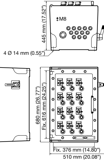
Layout Panel F
