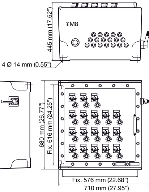
Layout Panel G
