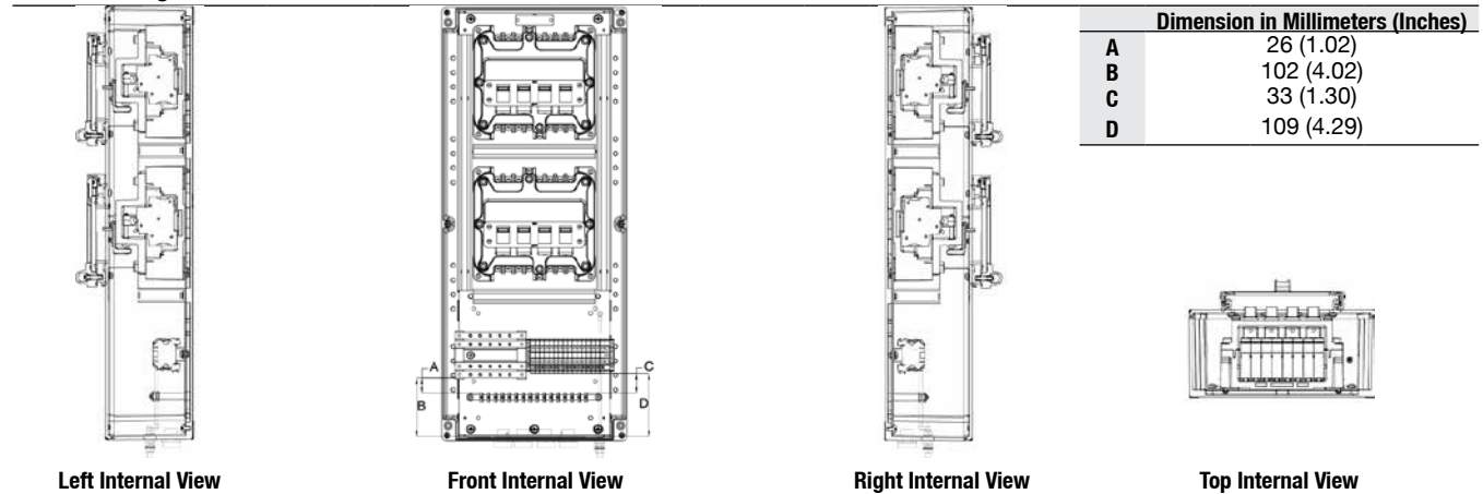
Panel Arrangement A
