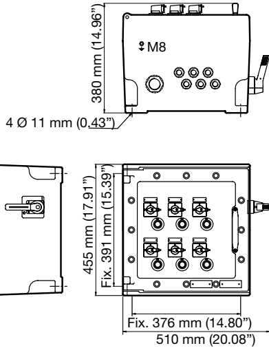
Layout Panel E
