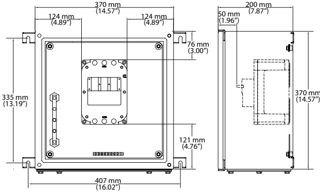
Size A 3-Pole Circuit QC
