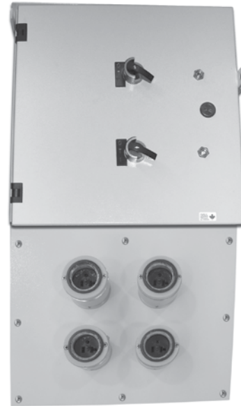
Shown with PlexPower™ External Actuating Enclosed Circuit Breaker and Receptacles
