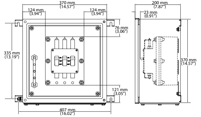
Size A 3-Pole Circuit F-Frame
