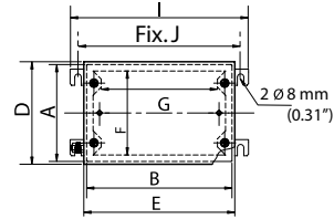
Mounting Bracket
