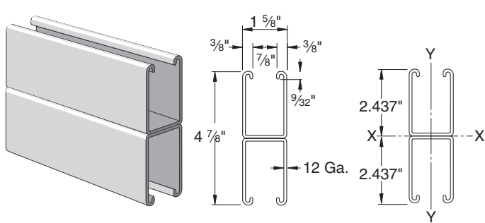
ELEMENTS OF SECTION – PS 150 2T3
