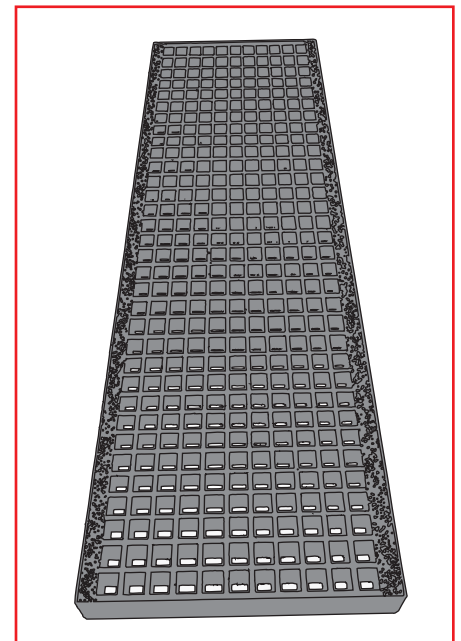
Panel size: 22-½" x 120" Approx. Weight: 105 lbs.
