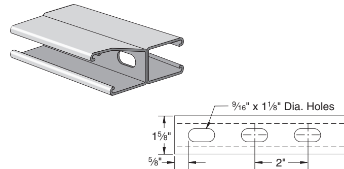
ELEMENTS OF SECTION – PS 150 2T3
