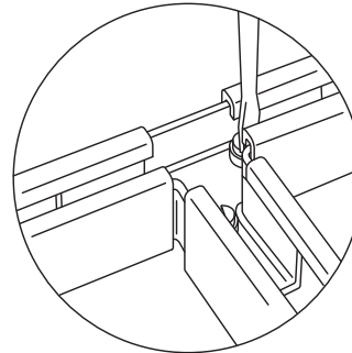
Channel should be supported a minimum of 12" from joiner.
