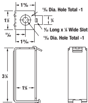
Hinged channel hanger for raceway channel.
