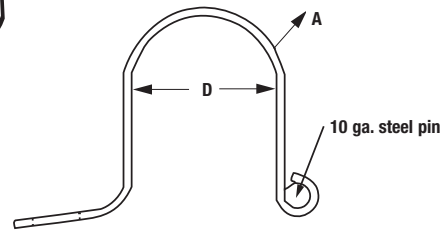
Straps are steel and have Galv-Krom® finish.
