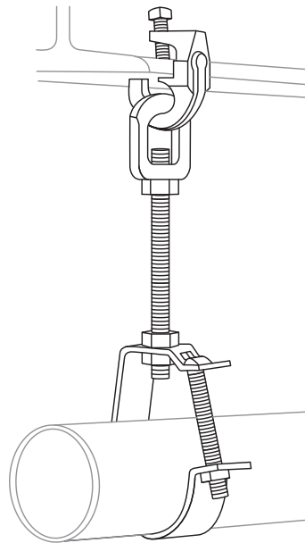
H-550 Swivel Beam Clamp supports pipe with C-711 hanger.
