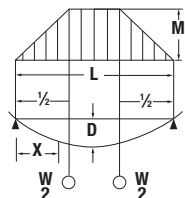
Beam supported at ends Two symmetrical concentrated loads W \text{ max.} = 2fS/a D \text{ max.} = Wa/12EI (\frac{1}{2}L^2 - a^2)
