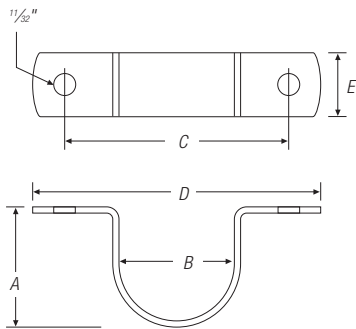
Holds pipe tight against mounting surface.
