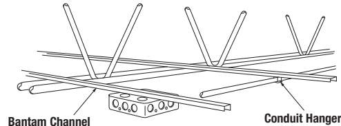
Typical mounting on bar joists
