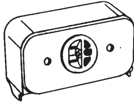
Complete unit including housing, standard single 3-wire, 15-amp. 125-volt NEMA ground receptacle and cover plate.
