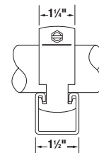
Pipe supported by C-149 lay-in hanger.
