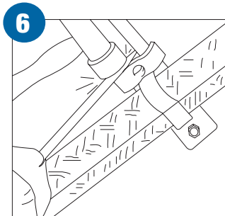
Drive locking device tight against cable strap. Tighten locking device screw.
