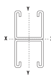
B-900-2A 1½" x 3" x 12 ga. steel
