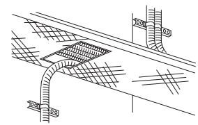
Armored Cable (Take-off from Cable Tray)
