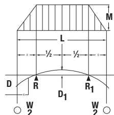
Beam continuous over two supports Two exterior symmetrical loads W \text{ max.} = 2fS/a D , distance a = Wa(3aL - 4a^2)/12EI D1 , distance L/2 - a = Wa(2-2a)^2/16EI
