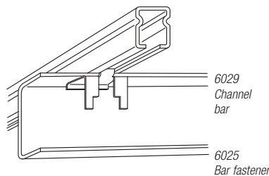
Cat. No. 6025 Secures channel to lathers channel or other ceiling-carrying channels.
