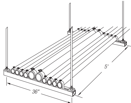
Trapeze application supporting multiple conduit runs.
