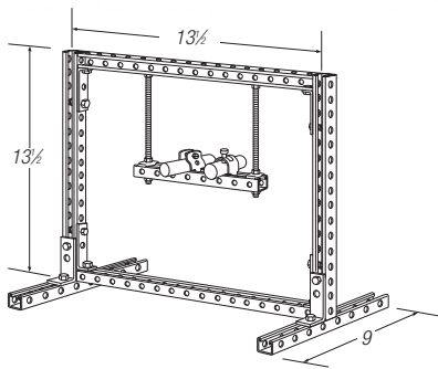
1 1/2" wide x 1 1/2" deep 7/8" continuous open slot 10 ft. and 20 ft. lengths
