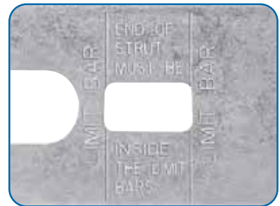
View window provides strut length safety zone for rough cuts versus precision cuts.
