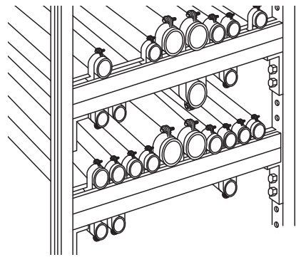
Steel beam mounting application. Aluminum straps with stainless steel hardware. Frame assembly carries multiple conduit runs.
