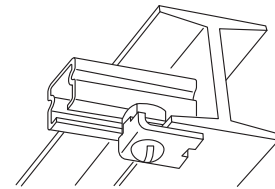
Cat. No. 6024 Secures channel to I-beams, angle iron or bar joists with flanges not exceeding 1/4" thickness.
