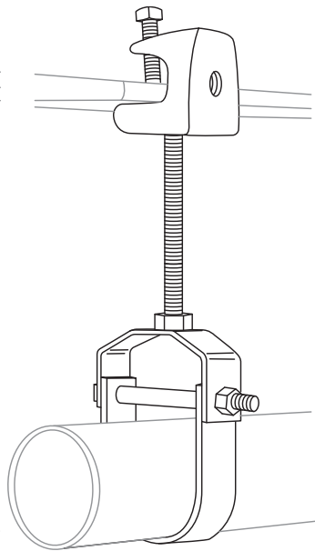
500 Series Beam Clamp supports pipe with C-710 clevis hanger.
