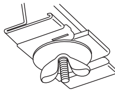
Cat. No. 6075 Mounts electrical fixtures to exposed grid acoustical ceilings. Fits 1/8" or 1" bar face. Load Rating: 100 lbs. Safety factor of 4. Furnished complete with cupped washer and wing nut.
