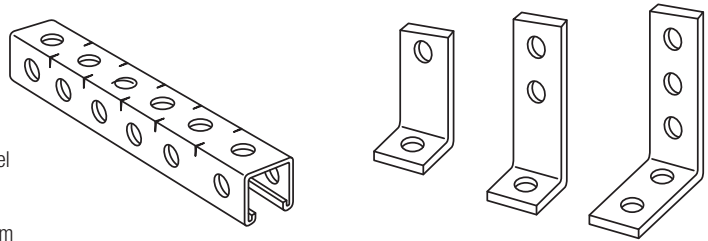
By simply stocking B-995 prepunched channel and three angle fittings, a great number of joints can be made.
