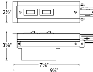
Recessed Flanged
