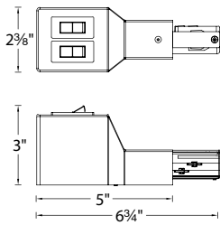
Surface Mount
