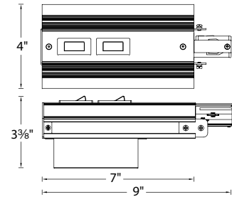
Recessed Flangeless
