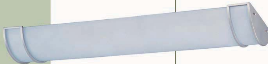
85538WTSN 3-Light Flush Mount Satin Nickel 48"L x 11.5"W x 4.5"Ext. 3 x 32w Med Bi Pin T8 Bulbs (Not Included) 8400 Rated Lumens CA T24
