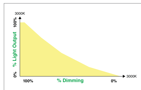
Traditional LED Dimming
