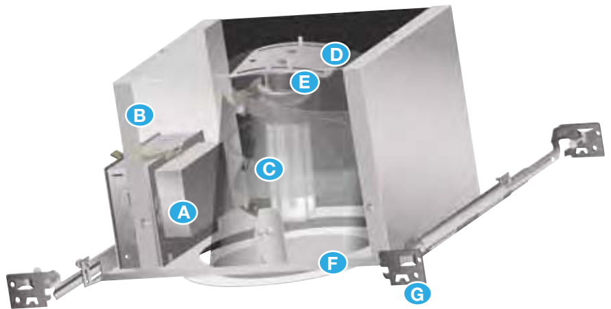
Illustrated here is the Juno ICPL926-42 housing with a 614W-WH trim.
