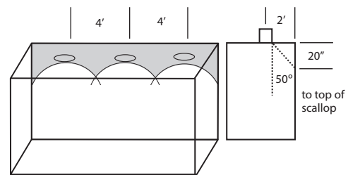
Well placed Light Scallops using 6" downlights
