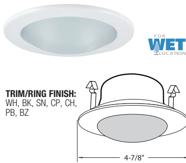
B439WH SMOOTH FROST DOME SHOWER LITE
