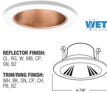
AF401W-WH SELF FLANGE BAFFLE
