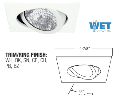
B442WH SQUARE PAR20 GIMBAL TRIM (30° TILT)
