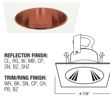
B444CL-WH SQUARE FROSTED LENS WITH REFLECTOR
