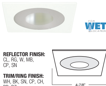
B444CL-WH SQUARE FROSTED LENS WITH REFLECTOR
