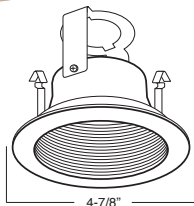
B496P-WH BAFFLE W/ ADJUSTABLE SOCKET BRACKET
