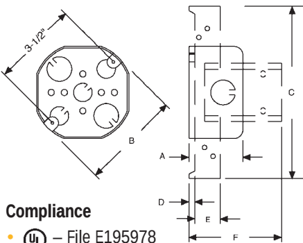
4" OCTAGON BOXES
