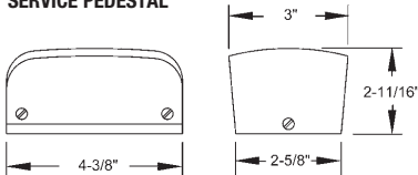
SERVICE PEDESTAL
