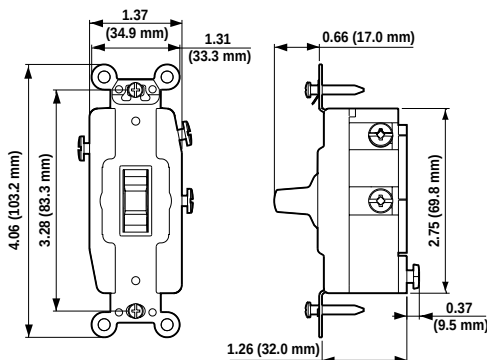
SINGLE-POLE, DOUBLE THROW Cat. No. 1256, 1257, 1281, 1285, 1287
