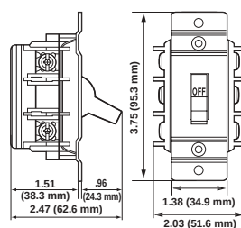
Cat. Nos. MS402, MS403
