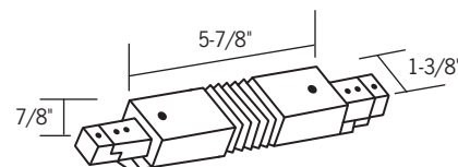
Flexible Connector: LA-203
