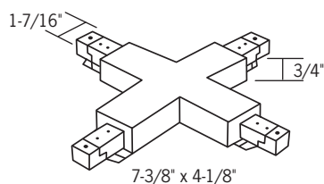
"X" Connector: LA-215
