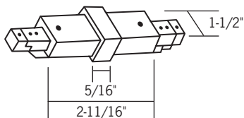
Mini-Connectors: LA-202
