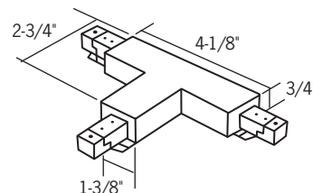
"T" Connector: LA-214
