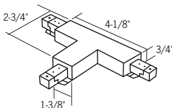
"T" Connector: LA-213
