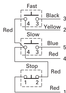
Figure A Pushbuttons
