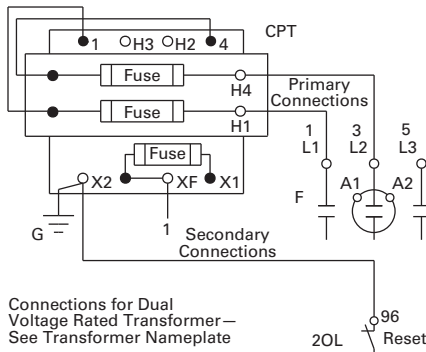
Figure 2 Control Circuit Transformer (If used) Remove Wire "C" if Supplied and Connect as Shown Below (All other wiring remains as shown in Figure 1)
