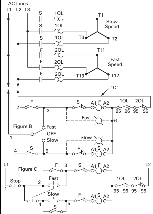
Starter Elementary Diagram
