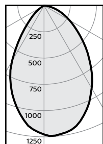
Candela Curve
