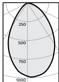
Candela Curve
