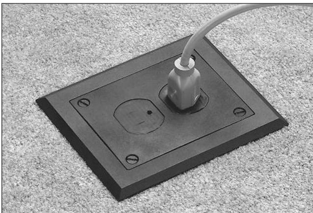
Source I Series Nonmetallic Single-Gang Flush Service Fitting.
