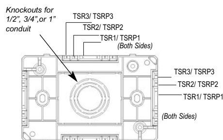
JB1, JB2 - SINGLE GANG
