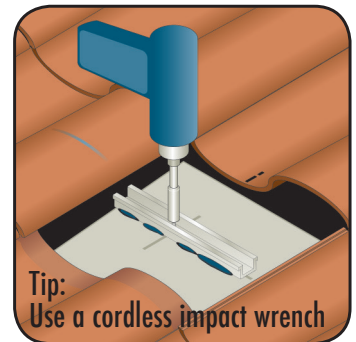
Step 6: Fasten lag screw until seated. Do not overtighten. The sealant should flow outward sealing any holes.
