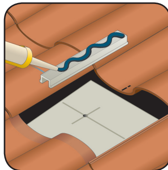
Step 5: Insert the lag bolt and washer through the TileTrac® and apply fresh compatible sealant to the base.
