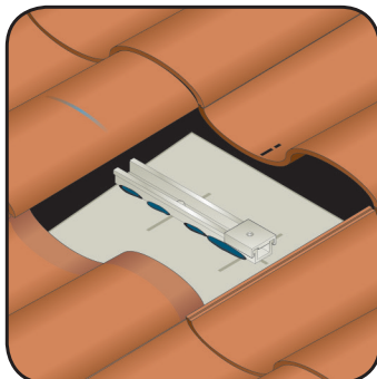
Step 7: After bolting the base to the roof, slide the upper carriage into the correct position under the crown of the tile. For Flat tile, slide the upper carriage near the middle of the tile.
