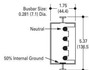
Typical Cross-Section
