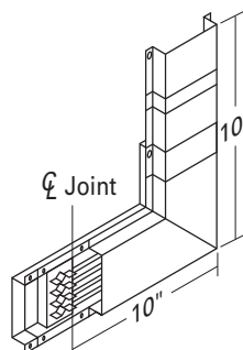
Upward Elbow
