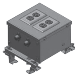
Fix-Mounted Duplex Receptacle
