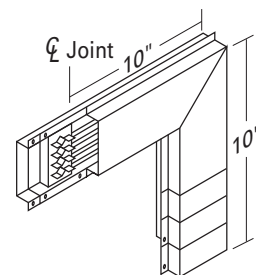
Downward Elbow
