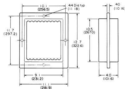
TWF10 (25 lbs.)
