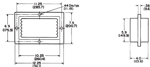
TWF6 (20 lbs.)
