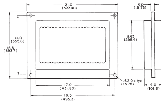
TWF20 (82 lbs.)
