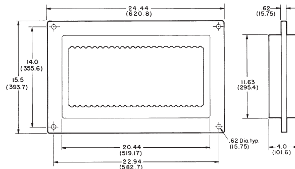
TWF24 (88 lbs.)
