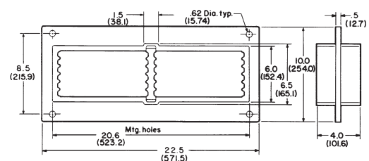
TWF12 (38 lbs.)
