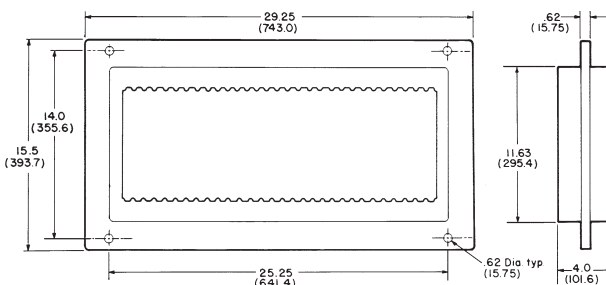
TWF30 (97 lbs.)
