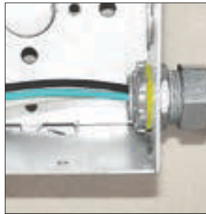
Built-in sealing gasket
