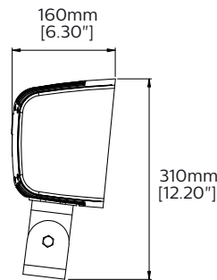
PFL80 Side
