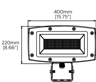
PFL150 Front
