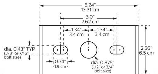
Trunion Mount Bolt Pattern
