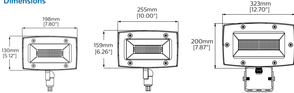
PFL20 Front
