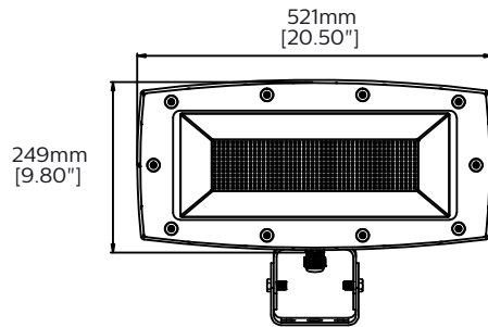
PFL300 Front
