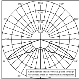
RESTL Test Report #: PLO9286-001A ARE-EDG-5S-**-06-E-UL-700-40K Initial Delivered Lumens: 14,123
