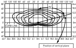
ARE-EDG-2MB-**-10-E-UL-525-40K Mounting Height: 25' (7.6m) A.F.G. Initial Delivered Lumens: 13,185 Initial FC at grade
