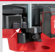
STEP 3: Cut is complete once moving jaw automatically releases back to home position
