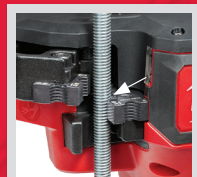
STEP 1: Hold rod against tool's fixed lower jaw
