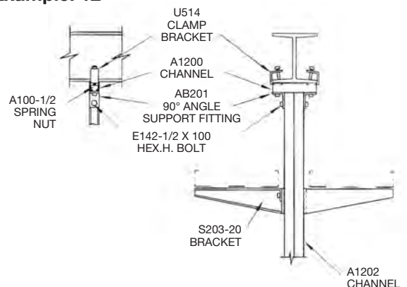
Brackets perpendicular to beam
