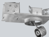
P8200-EB 6" HID Pro-Optic Housing One ED17 or PAR30L MH lamp, each 70w max.
