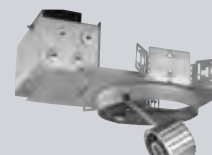
P8201-EB 6" HID Pro-Optic Housing One ED17 MH lamp, each 100w max.
