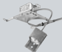
P63-EB Recessed Two Quad 4-pin Comp. Fl. lamps, each 13w.
