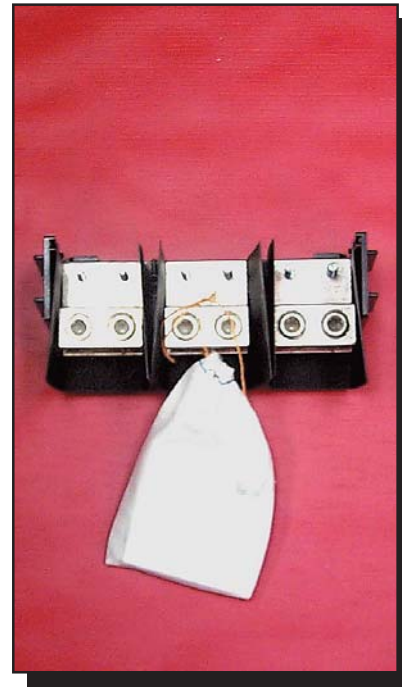
Catalog # 020-509-01-00-0 MPAP, MPRV & Unicorn MPP lug landing assembly with grounding kit
