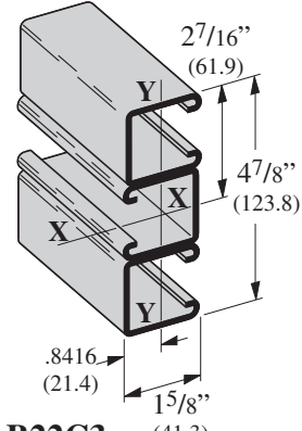
B22C3 Wt. 5.70 Lbs./Ft. (8.48 kg/m)
