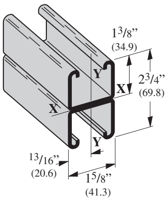
B32A Wt. 3.40 Lbs./Ft. (5.06 kg/m)
