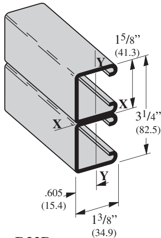
B32B Wt. 3.40 Lbs./Ft. (5.06 kg/m)
