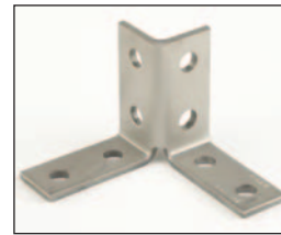
B121 8-Hole Double Corner Connection
