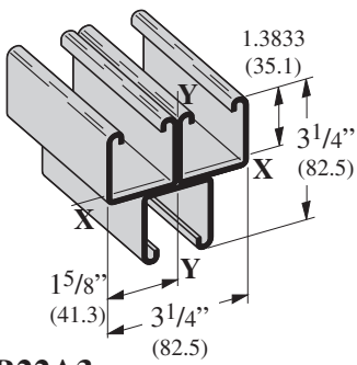
B22A3 Wt. 5.70 Lbs./Ft. (8.48 kg/m)
