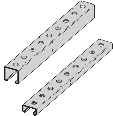
BK_H112 CHANNEL WITH 9/16" HOLES ON 1 1/2" CENTERS & CUTTING MARKS ON 1 1/2" CENTERS Pg. 42
