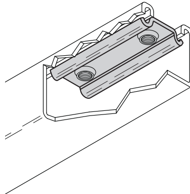
DCN3/8 CONVEYOR NUT Pg. 52
