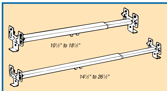
Foot straightened gauges for 1/2"-deep box with cover or 2 1/8"-deep box without cover. With foot broken off gauges for shallow pan box.
