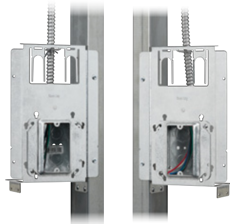
Can be mounted either left or right of the stud
