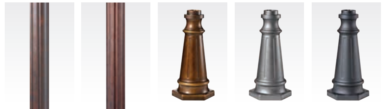
7' Post WOBZ FINISH: Woodland Bronze Extruded Aluminum Wall Thickness: 2.7mm Diameter: 3" 7' Post WP FINISH: Weathered Patina Extruded Aluminum Wall Thickness: 2.7mm Diameter: 3" Post Base ASTB FINISH: Astral Bronze Die Cast Aluminum H: 19 1/2" D: 10" Post Base BB FINISH: Burnished Bronze Die Cast Aluminum H: 19 1/2" D: 10" Post Base BK FINISH: Black Die Cast Aluminum H: 19 1/2" D: 10"
