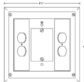
60° Angle Plates
