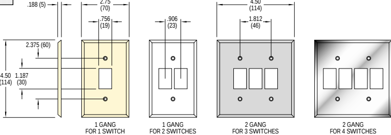
ALL DIMENSIONS ARE TYPICAL inches (millimeters)
