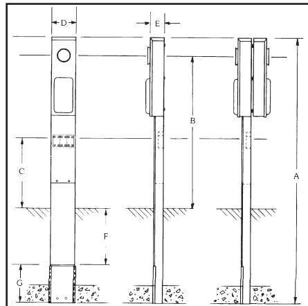
Single Head Post
