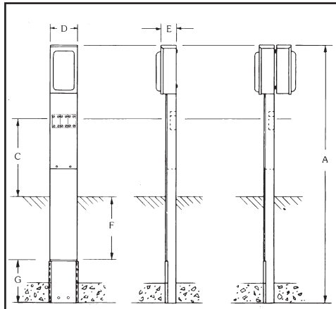
Single Head Post
