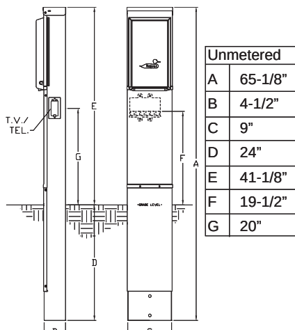
U041CP6031- see pg. 78
