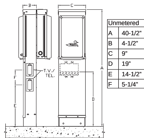
U075CB4031- see pg. 80
