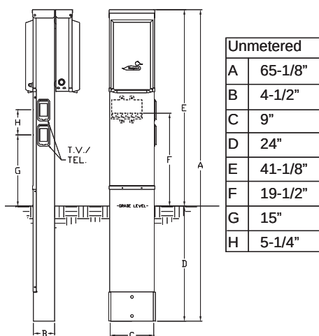
U075CB6031- see pg. 80
