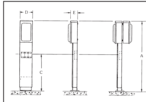
Single Head Post
