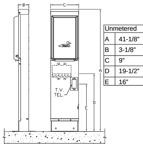
U004CP4031- see pg. 78
