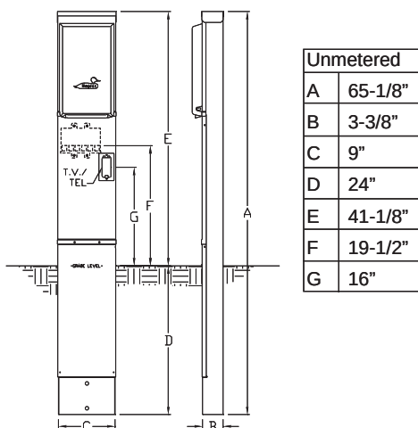
U075CP6031- see pg. 78
