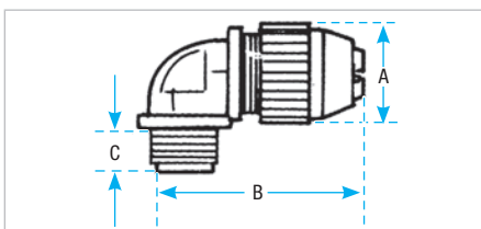
90° angle, standard size body.
