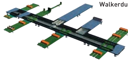
Walkerduct Layout with Junction Boxes
