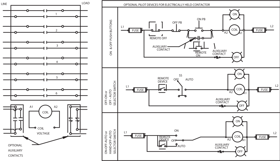
CR463L Electrically Held
