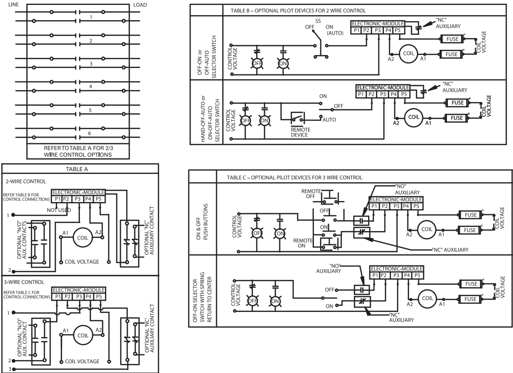
CR463M Mechanically Held
