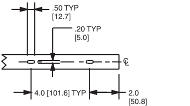
Mounting Hole Dimensions For .5", .75", 1", and 1.5" wide duct.
