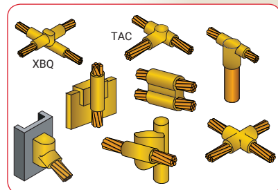
Cadweld Connections
