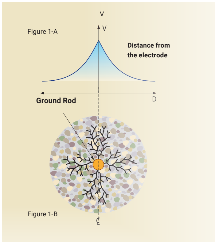
Figure 1-B illustrates current flow from the injection point of a single ground electrode. As current flows out from the central injection point, a voltage gradient on the ground surface around the electrode is produced. This gradient levels off to a plateau at some distance from the electrode, as seen in Figure 1-A. The impedance seen by the current is determined by the soil particles in direct contact with the surface of the rod, and by the general impedance of the soil.
