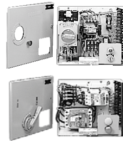
Motor Control Center Bucket Retrofits
