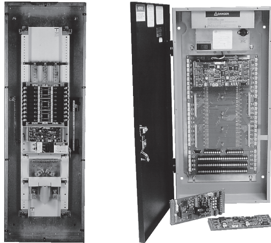
Pow-R-Command Lighting Control
