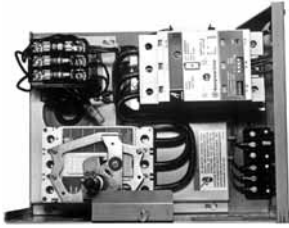
GE770 Unit Retrofitted with Advantage and HMCP
