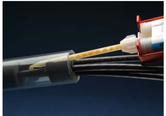
The FST Sealant comes in a side-by side (two plunger) system, as shown above, or a caulking style (one plunger) tube. Both options allow multiple use. Mixing is done in the nozzle as the sealant is injected.
