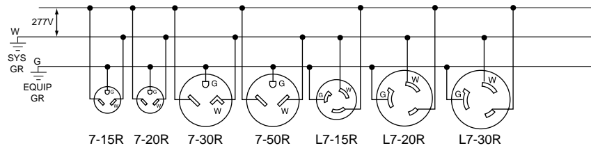
277V AC — 2-POLE, 3-WIRE GROUNDING
