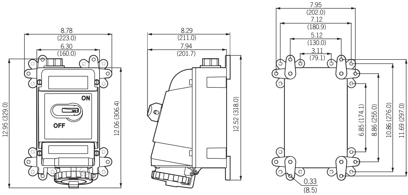
20 AMP & 30 AMP FUSED AND NON-FUSED
