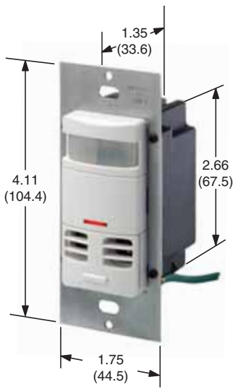
OSSMT-MD Multi-Tech Sensor
