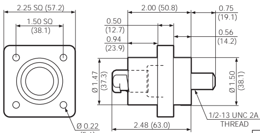
MALE THREADED STUD PANEL RECEPTACLE
