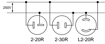
250V — 2-POLE, 2-WIRE
