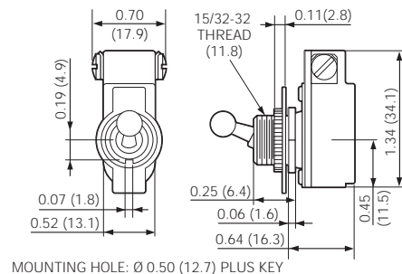
735—SINGLE POLE TOGGLE SWITCH
