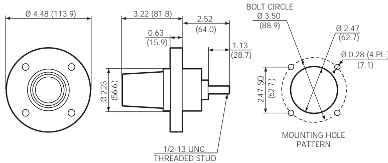
90° FEMALE PANEL RECEPTACLE THREADED STUD
