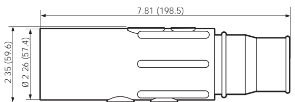
MALE VULCANIZED PLUG—CRIMPED
