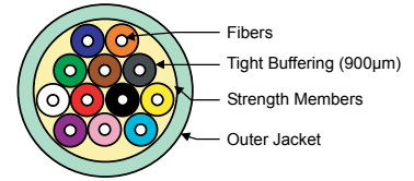
12-Fiber Cable Cross Section
