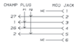
C. 2-Pair 6-Position
