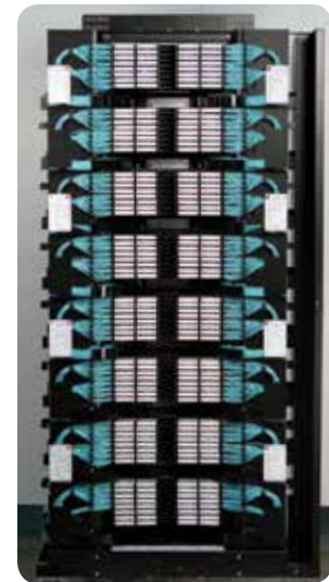
Q-Frame loaded with (8) 4RU Quareo chassis and (64) Quareo LC-to-MPO blades (3,072 LC fiber terminations)
