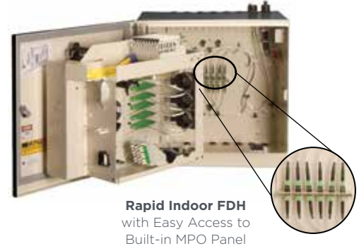
Rapid Indoor FDH front panel
