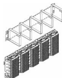
35.5" high volume cable manager with 5 rings, shown mounted above 5 Type 105 mounting brackets
