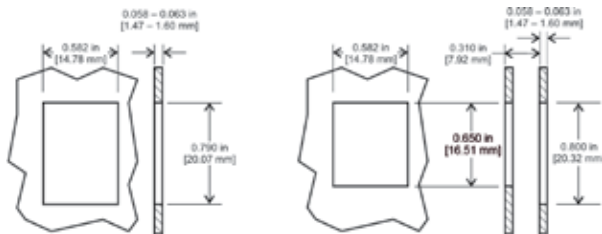
Suggested Single Panel Cutout
