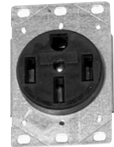
708767-MO 50 amp receptacle NEMA 1450
