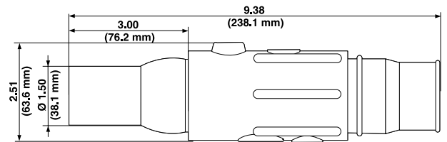
Female Detachable Plug – Double Set Screw
