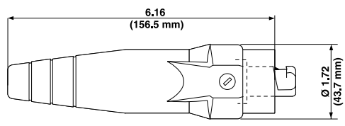
Male Detachable Plug – Single Set Screw
