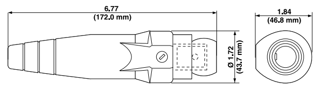
Female Detachable Plug – Single Set Screw
