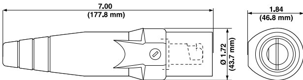
Male Detachable Plug – Crimped
