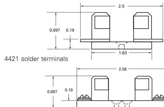
4515 with screw terminals
