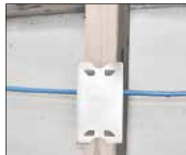
PROTECT CABLES FROM DRYWALL SCREWS
