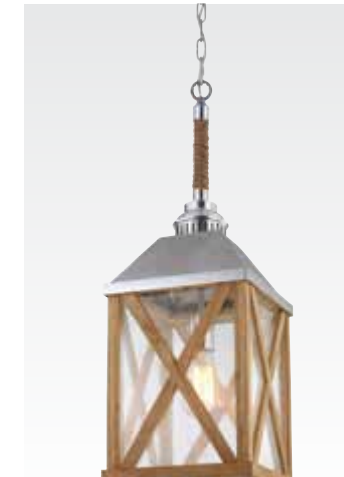
F2956/1 NO H: 18.5" D: 9.75" 5' Chain (1) 100W Medium Antique Bulb Recommended Lumière
