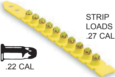
POWER DRIVEN
