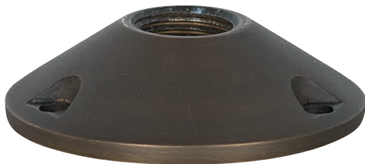
B2012 Flat Base Cast Brass Matte Bronze Finish 2.75"D Center Hole 1/2"NPT Female
