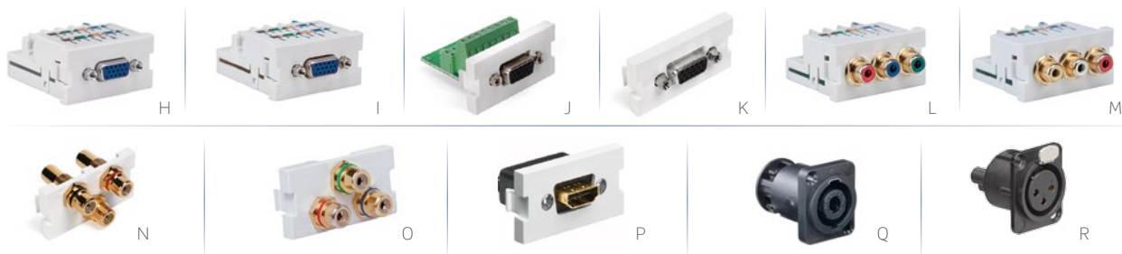
Multimedia Outlet System AV connector modules (All modules are 1-unit high unless noted otherwise)
