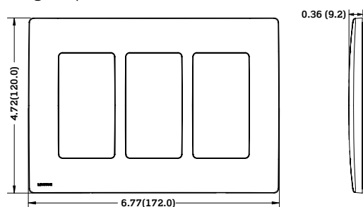
3-Gang Wallplate
