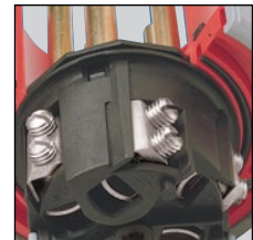
Terminal Screws
