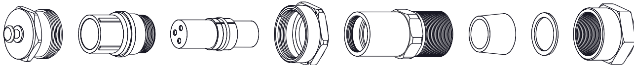
Environmental Cover
