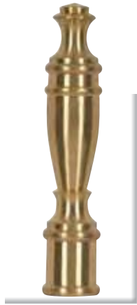
90-1731 Large Spindle Finial 2 3/8" Height - 1/4-27 Polished Brass
