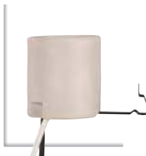
80-1220 Snap-In Socket Bracket Extends 1" from End of Socket 12" AWM B/W Leads 150°C 660W-250V
